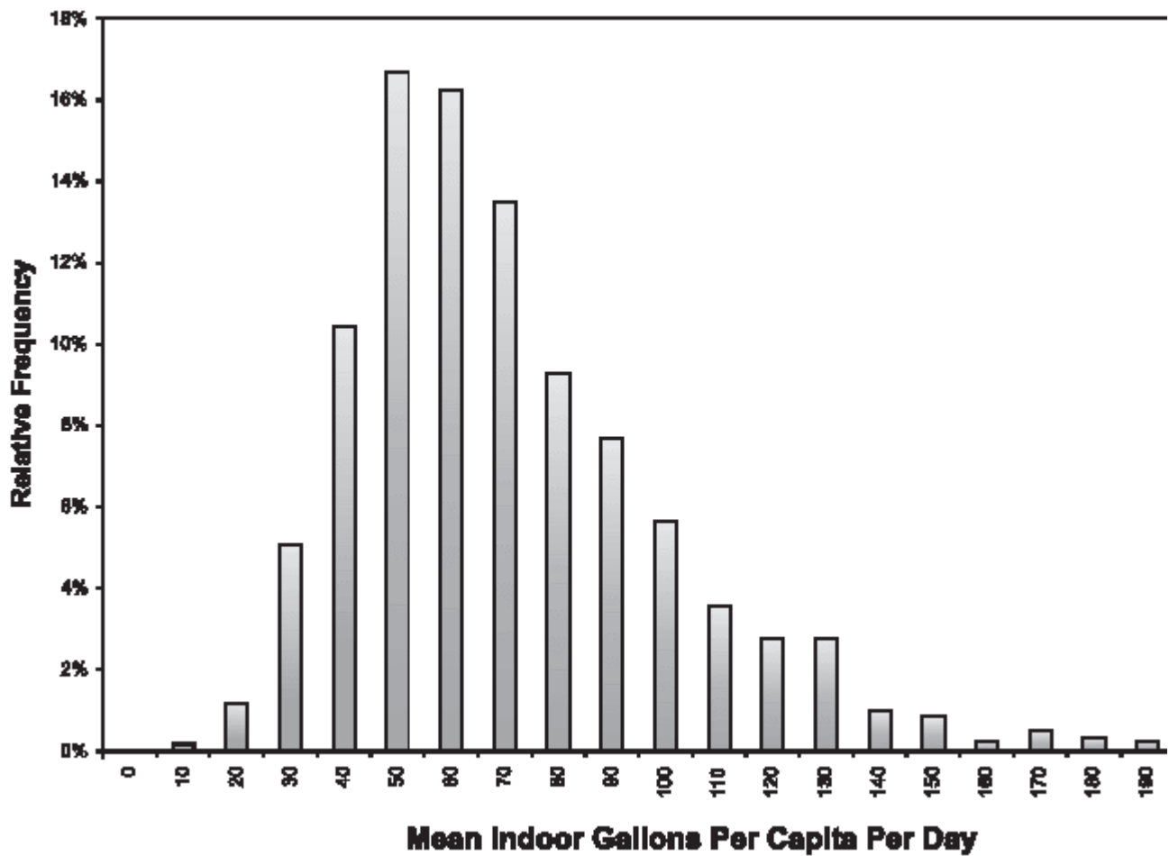
Figure 3-1. Distribution of mean household daily per capita indoor water use for 1,188 data-logged homes
