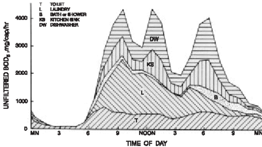
Figure 3-5. Average hourly distribution of total unfiltered BOD 5
