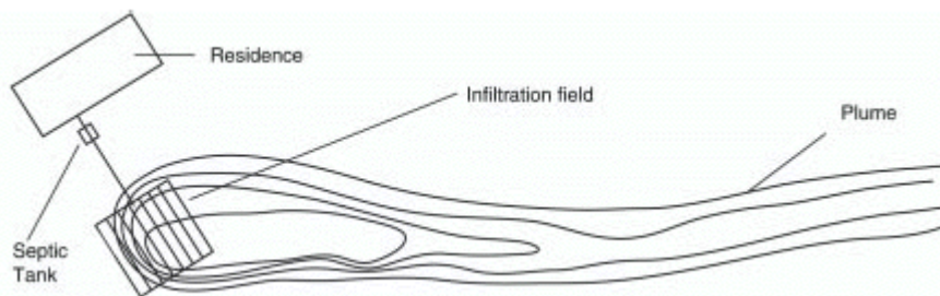
Figure 3-9. An example of effluent plume movement
