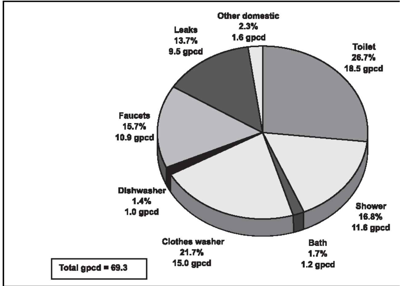
Figure 3-2. Indoor water use percentage, including leakage for 1,188 data logged homes a
