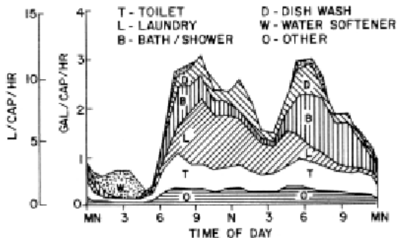
Figure 3-4. Peak wastewater flows for single-family home
